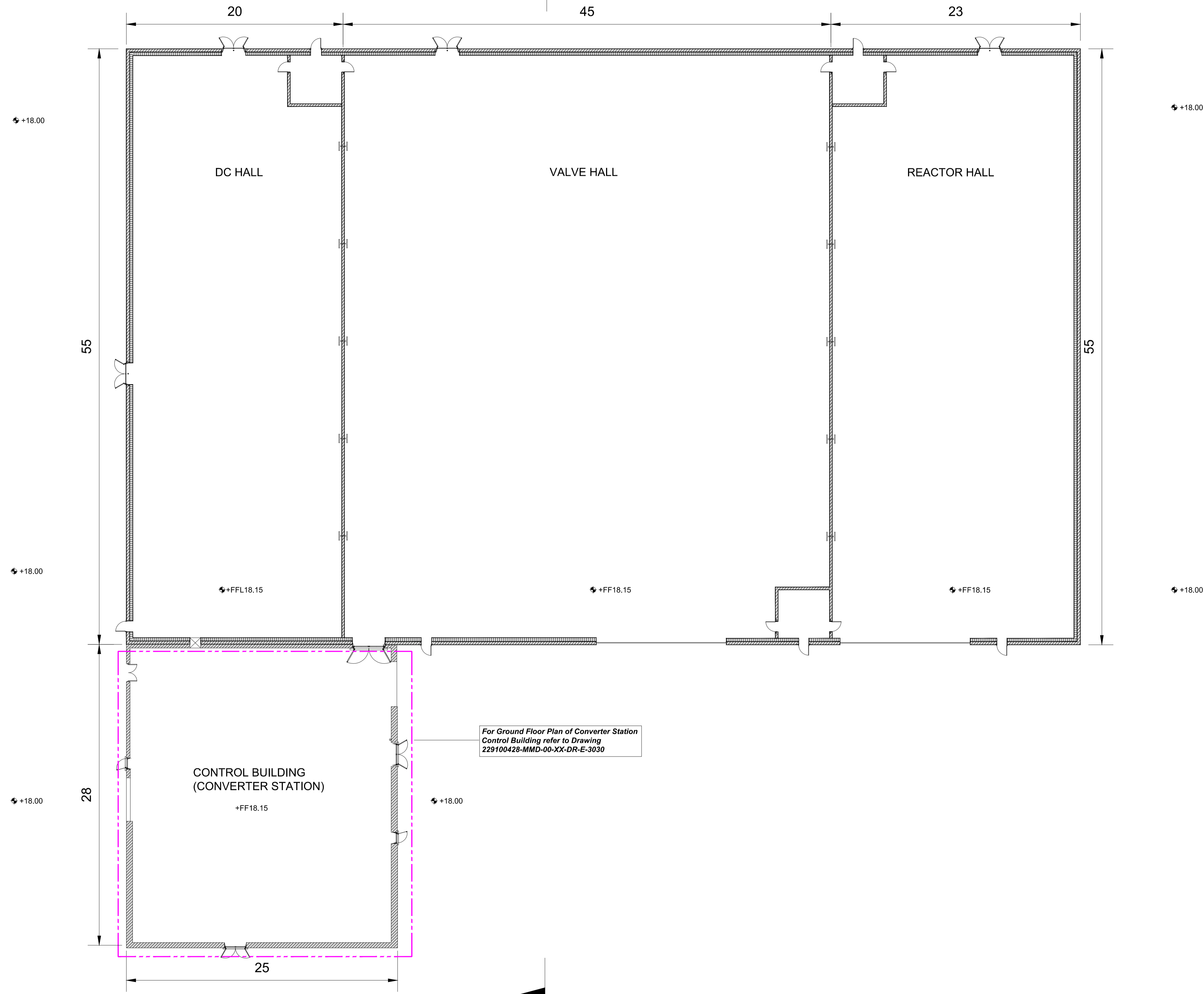
Ground Floor Plan 1:200
